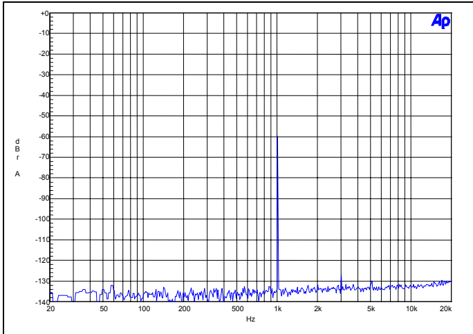
Figure 4 - FFT -60dB, 1kHz Output, DDX mode
