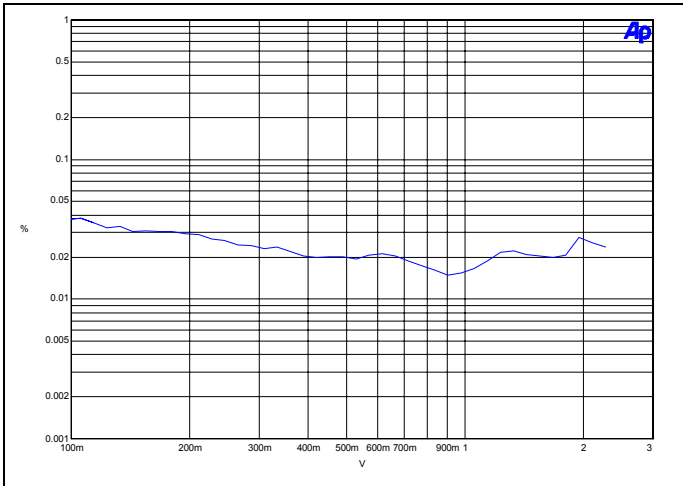
Figure 14 - THD vs. Voltage RMS , 1kHz
