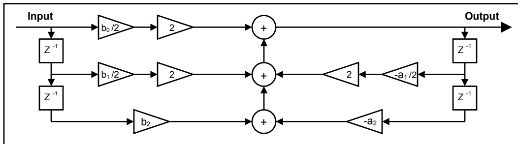
Figure 23 - Biquad Filter
