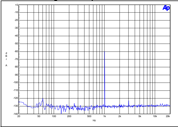
Figure 12 - FFT -60dB, 1kHz Output
