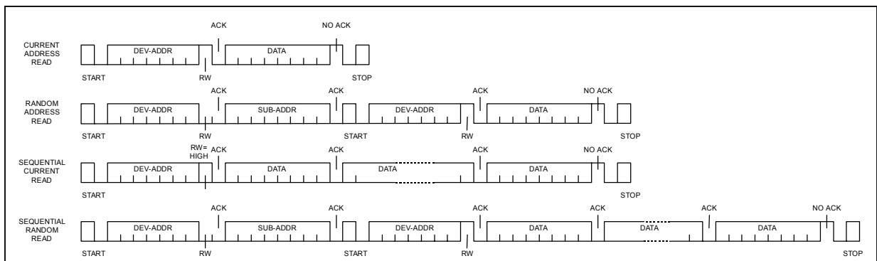
Figure 17 - I 2 C Read Procedure
