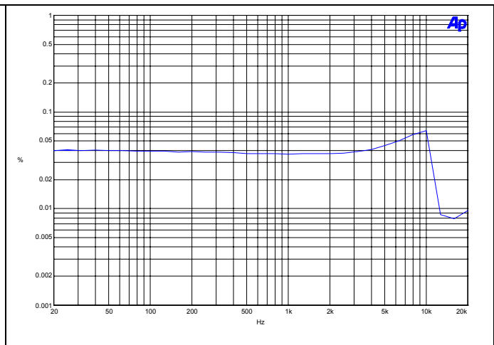
Figure 7 - THD vs. Frequency, 1W
