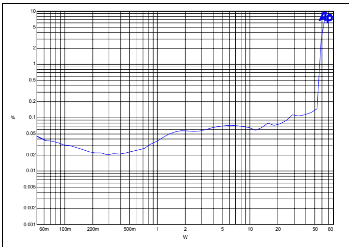
Figure 6 - THD vs. Power, 1kHz
