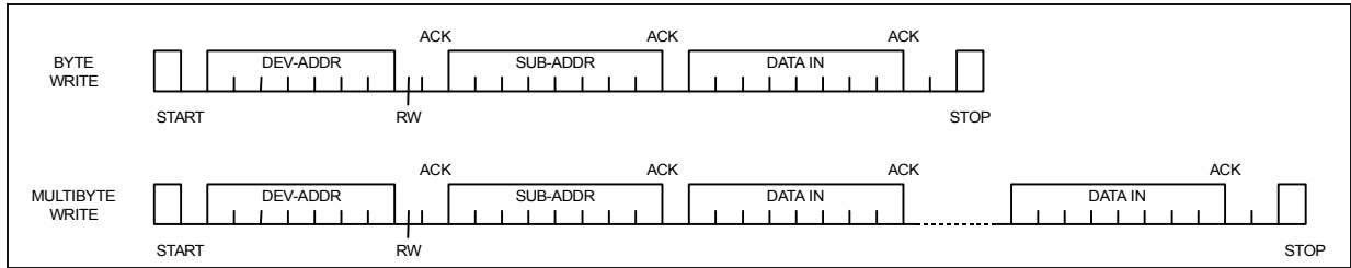
Figure 16 - I 2 C Write Procedure
