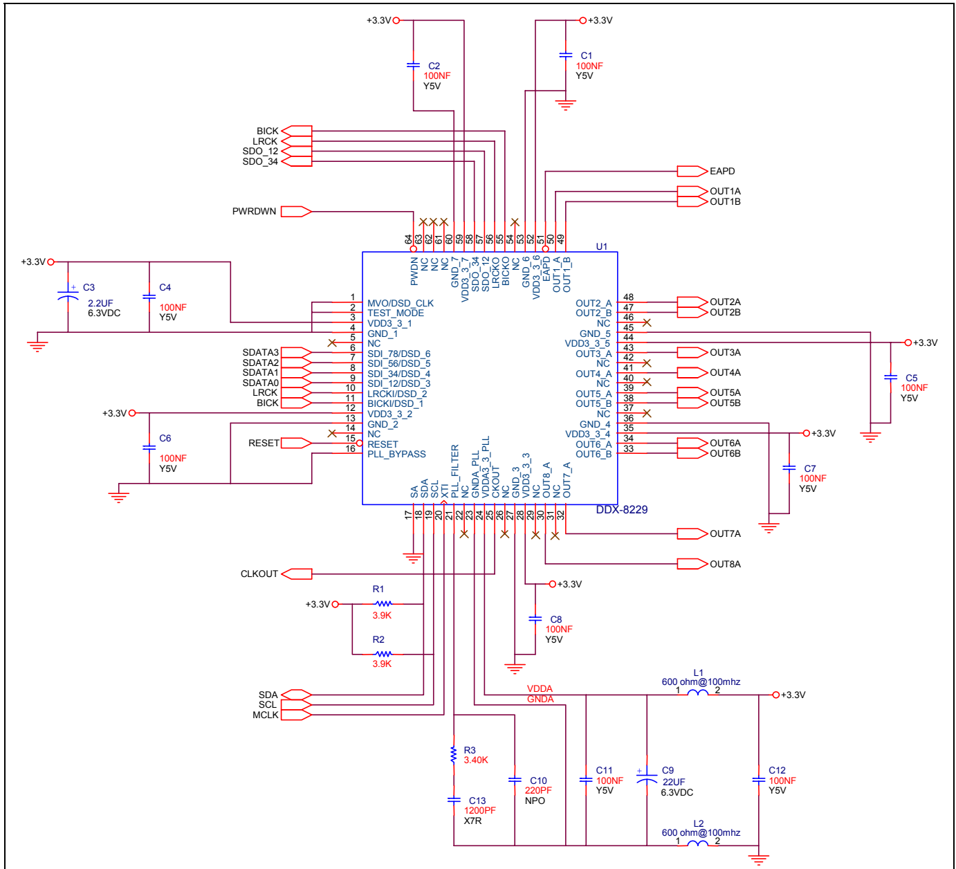
Figure 25 - Schematic Diagram.
