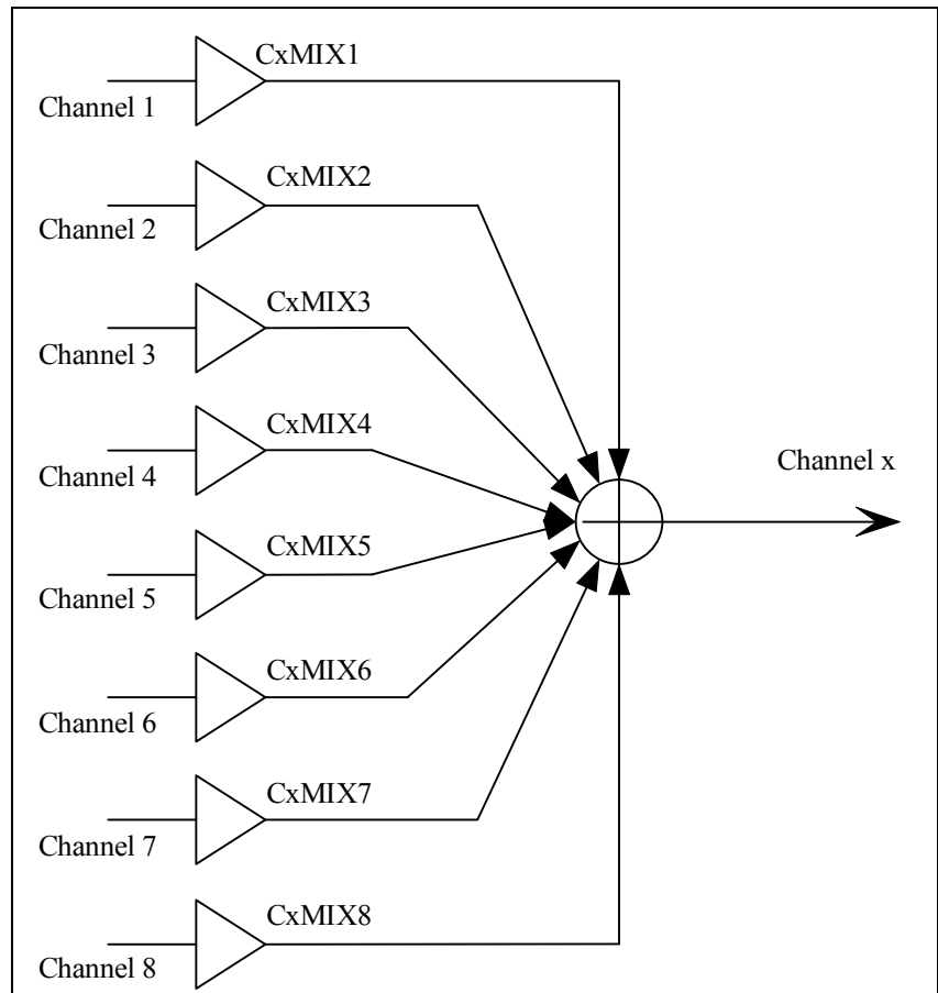
Figure 24 - Mix Block Diagram
